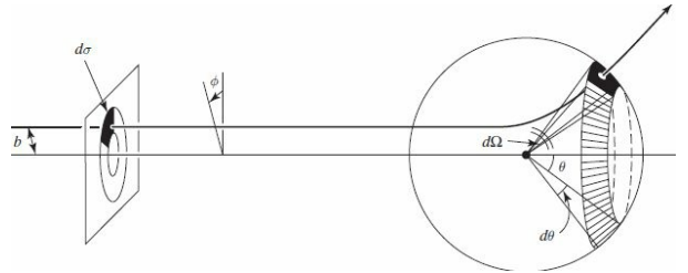
Fig. 2: Scattering of waves; an incoming plane wave generates an outgoing spherical wave.
