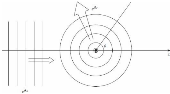
Fig. 2: Scattering of waves; an incoming plane wave generates an outgoing spherical wave.
